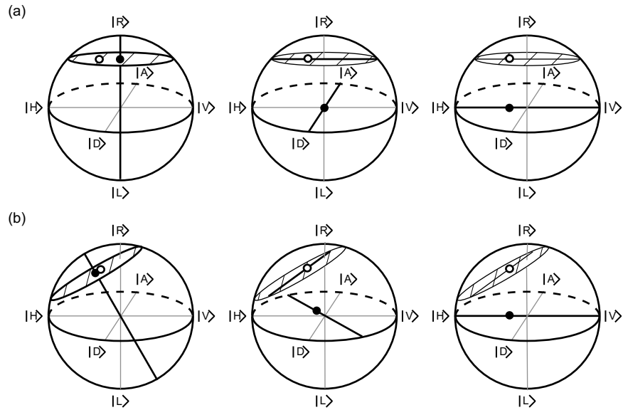
Figure 2: A sequence of three linearly independent measurements isolates a single quantum state in Hilbert space (shown here as an open circle in the Poincaré sphere representation). The first measurement isolates the unknown state to a plane perpendicular to the measurement basis. Further measurements isolate the state to the intersections of non-parallel planes, which for the second and third measurements correspond to a line and finally a point. The black dots shown correspond to the projection of the unknown state onto the measurement axes, which determines the position of the aforementioned planes. (a) A sequence of measurements along the right-circular, diagonal, and horizontal axes. (b) A sequence of measurements on the same state taken using non-orthogonal projections: elliptical light rotated 30^\circ from H towards R, 22.5^\circ linear, and horizontal. Taken from (Altepeter et al., 2004).
