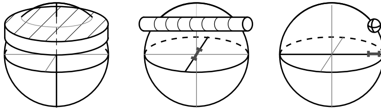
Figure 7: Isolation of a quantum state through inexact measurements. Although a series of real measurements (those with uncertainties) will never be able to exactly isolate an unknown quantum state, they can isolate it to a region of Hilbert space that is far more likely than any other region to contain the unknown state. Consider a series of three measurements, each containing counting errors, along orthogonal axes. From left to right, the area of Hilbert space containing the unknown state is truncated from a one-dimensional Gaussian probability distribution (the disk in the left figure) to a two-dimensional Gaussian (the cylinder in the middle figure) and finally to a three-dimensional Gaussian (the ball in the right figure). This results in an ‘error ball’ which approximates the position of the unknown state. The global maximum, however, can often be outside allowed Hilbert space (outside the Poincaré sphere), which is one reason a maximum likelihood technique must be used to search over only allowed quantum states.
