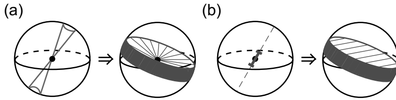
Figure 6: Graphical representation of errors in a single-qubit tomography. (a) Basis errors. Errors in the setting of measurement apparatus can result in an accurate measurement being taken in an unintended basis. Shown graphically is the effect that an uncertainty in the measurement basis can have on the reconstruction of a state. Instead of a single axis on the Poincaré sphere, the possible measurement axes form uncertainty cones touching at the center, since all possible measurement axes pass through the origin. This uncertainty in axis is then translated into an uncertainty in the state (shown on the right). Instead of isolating the state to a plane, all possible measurement axes trace out a volume with large uncertainty near the surface of the sphere and low uncertainty near the center. (b) Counting errors. Even if the measurement basis is exactly known, only a limited number of qubits can be measured to gain an estimate of a state's projection onto this axis (taken directly from the probability of a successful measurement). This uncertainty results in an unknown state being isolated to a one-dimensional gaussian (approximately) in three-dimensional space, rather than to a plane.
