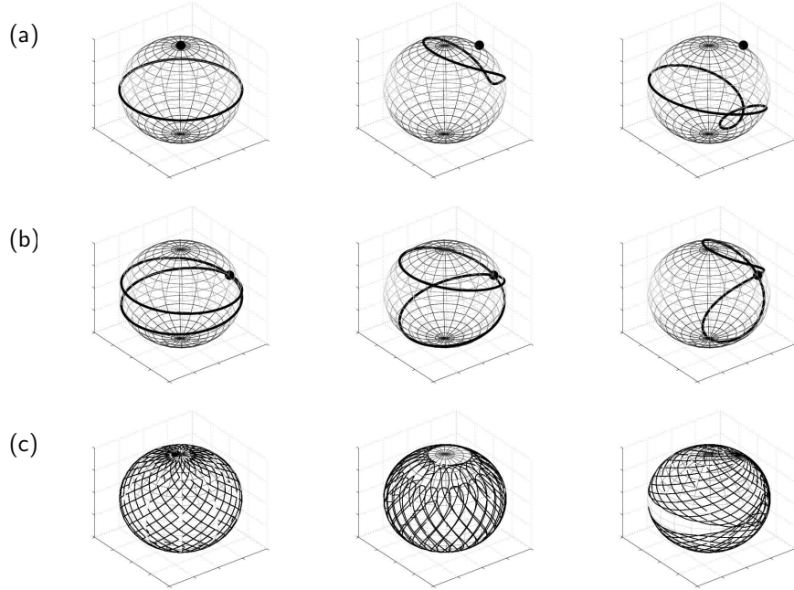
Figure 4: Possible projectors simulated by waveplates and a stationary polarizer, graphically shown on Poincaré spheres. (a) WP_1 , depending on its orientation, can rotate an incoming state into a variety of possible output states. Shown here on three Poincaré spheres are an initial incoming state (represented by a solid dot) and the set of all output states that WP_1 can rotate it into (represented by a dark band on the surface of the sphere). From left to right, the spheres depict |R\rangle transformed by a \frac{\pi}{2} -waveplate, |\gamma\rangle = \cos(\frac{\pi}{8})|H\rangle + i\sin(\frac{\pi}{8})|V\rangle transformed by a \frac{\pi}{3} -waveplate, and |\gamma\rangle transformed by a \frac{2\pi}{3} -waveplate. (b) WP_2 , depending on its orientation, can rotate a variety of states into the target state |H\rangle . Shown here from left to right are the states able to be rotated into |H\rangle by a \frac{11\pi}{12} -waveplate, a \frac{3\pi}{4} -waveplate, and a \frac{\pi}{2} -waveplate. (c) The possible projectors able to be produced by two waveplates and a horizontal polarizer. A series of arcs blanketing the Poincaré sphere show the areas of the sphere representing achievable projectors for each waveplate combination. From left to right, the spheres show the states (in this case, all of them) accessible from an ideal QWP and HWP, the states accessible using \frac{\pi}{3} - and \frac{11\pi}{12} -waveplates (groups of states near the poles are inaccessible), and the states accessible using \frac{\pi}{3} - and \frac{3\pi}{5} -waveplates (states on the equator are inaccessible). Note that the spheres shown in (c) are not simply combinations of the spheres above it, but include retardance values chosen to illustrate the possible failure modes of imperfect waveplates.
