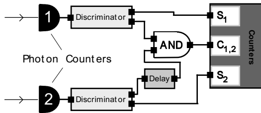
Figure 5: A simple diagram of the electronics necessary to operate a coincidence-based photon counting circuit. While this diagram depicts a two-detector counting circuit, it is easily extendible to multiple detectors; by adding additional detectors each fed into a discriminator and a fan-out, we gain the signals necessary for one singles counter per detector and an AND gate for each pair of detectors capable of recording a coincidence.
