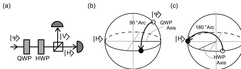
Figure 3: A quarter-waveplate (QWP), half-waveplate (HWP), and polarizing beam splitter (PBS) are used to make an arbitrary polarization measurement. Both a diagram of the experimental apparatus (a) and the step-by-step evolution of the state on the Poincaré sphere are shown. (b) The quarter-waveplate rotates the projection state (the state we are projecting into, not the incoming unknown state) into the linear polarization plane (the equator). (c) The half-waveplate rotates this linear state to horizontal. The PBS transmits the projection state (now |H\rangle ) and reflects its orthogonal complement (now |V\rangle ), which can then both be measured.
