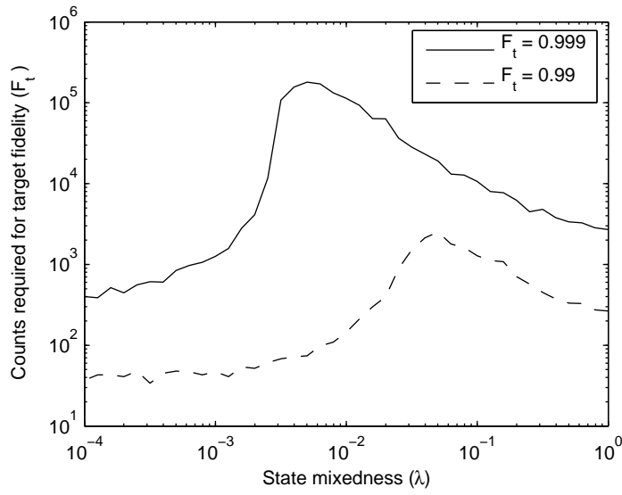
Figure 8: This plot shows the counts per measurement for a 4-detector system using the minimum nine measurement settings to achieve either a 99% (dotted line) or a 99.9% (solid line) target fidelity ( F_t ) with the ideal state. These results used Monte Carlo simulations on the Werner State (1 - \lambda)\hat{\rho}_{\frac{1}{\sqrt{2}}|HH+VV\rangle} + \lambda\frac{I}{4} , for a range of values of \lambda .
