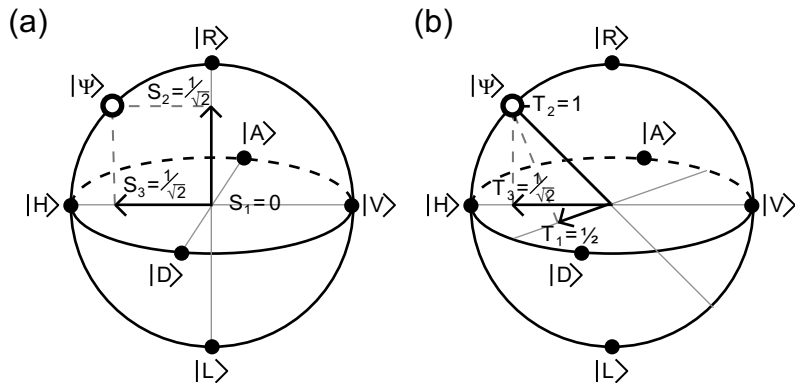
Figure 1: The Poincaré (or Bloch) sphere. Any single-qubit quantum state \hat{\rho} can be represented by three parameters T_i = \text{Tr}\{\hat{\tau}_i \hat{\rho}\} , as long as the operators \hat{\tau}_i in addition to the identity are linearly independent. Physically, the T_i parameters directly correspond to the outcome of a specific projective measurement: T_i = 2P_i - 1 , where P_i is the probability of success for the measurement. The T_i may be used as coordinates in 3-space. Then all 1-qubit quantum states fall on or within a sphere of radius one. The surface of the sphere corresponds to pure states, the interior to mixed states, and the origin to the totally mixed state. Shown is a particular pure state |\psi\rangle , which is completely specified by its projection onto a set of non-parallel basis vectors. (a) When \hat{\tau}_i = \hat{\sigma}_i (the Pauli matrices), the basis vectors are orthogonal, and in this particular case the T_i are equal to the S_i , the well known Stokes parameters, corresponding to measurements of diagonal ( S_1 ), right-circular ( S_2 ), and horizontal ( S_3 ) polarizations. (b) A non-orthogonal coordinate system in Poincaré space. It is possible to represent a state using its projection onto non-orthogonal axes in Poincaré space. This is of particular use when attempting to reconstruct a quantum state from mutually biased measurements. Shown here are the axes corresponding to measurements of 22.5^\circ linear ( T_1 ), elliptical light rotated 22.5^\circ from H towards R ( T_2 ), and horizontal ( T_3 ). Taken from (Altepeter et al., 2004).
